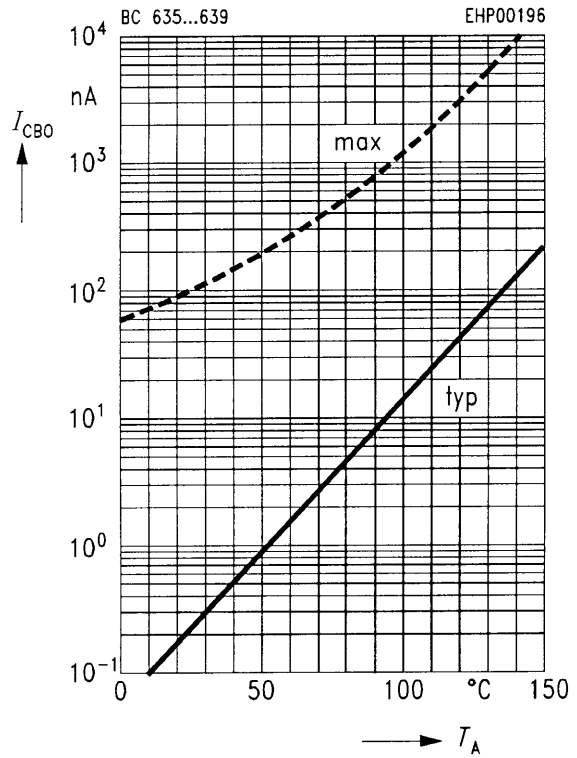
Collector cutoff current I_{CB0} = f(T_A) V_{CB} = 30 V
